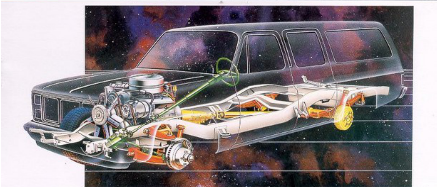
Cutaway of Sierra Classic 2-WD Suburban
